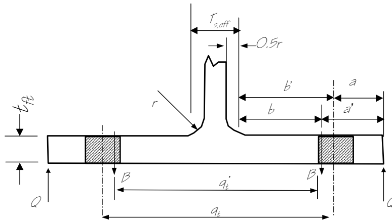
Figure 3-21 Geometry for Prying Forces and Bending of T-Section Flanges
